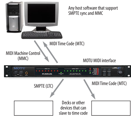
Figure 8-1: Your MOTU interface (a MIDI Express XT in this example) can serve as a time code “hub” while you control it from your sequencer via MMC transport commands.
