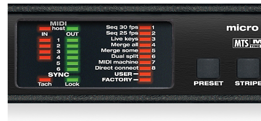
Figure 6-1: The eight factory presets on the front panel of the Express XT and micro express.
