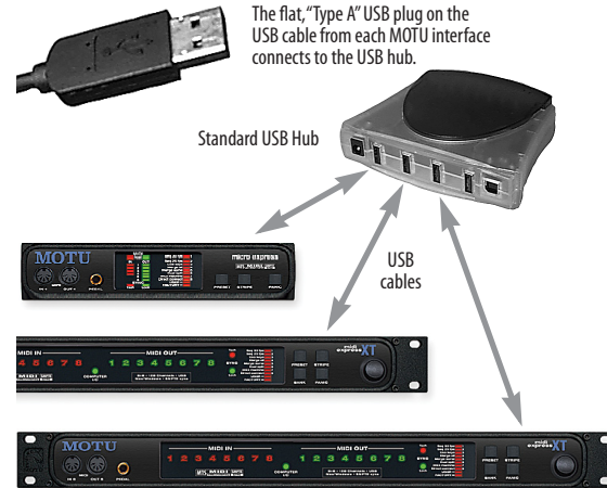
Figure 2-8: An inexpensive, standard USB hub allows you to connect multiple MOTU USB MIDI interfaces. You can even mix and match different models of MOTU USB MIDI interfaces, using the combination that best suits your needs for synchronization, number of MIDI ports, etc.
