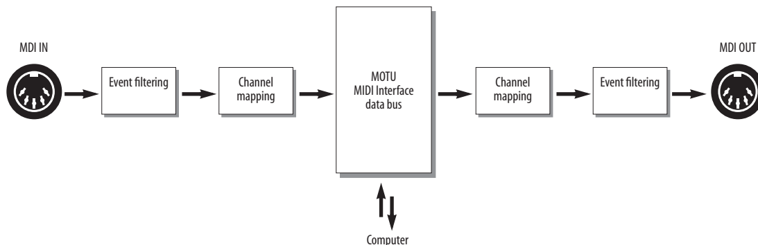
Figure 4-3: The path that MIDI data takes through a MOTU Express XT or micro express. Other MOTU interfaces do not provide MIDI processing.
