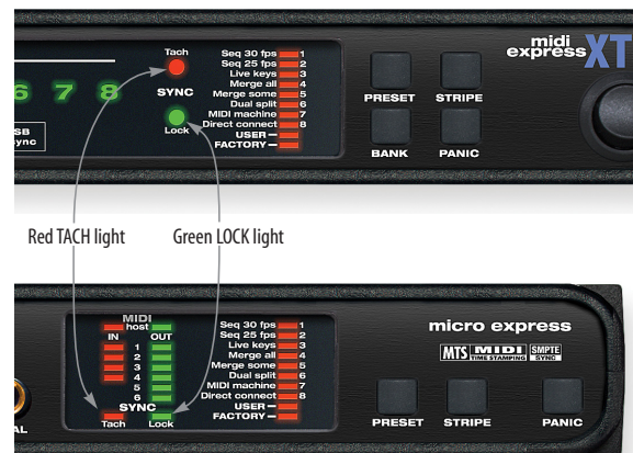
Figure 7-2: Converting time code. When your Express interface converts incoming time code, the red TACH light blinks, the green LOCK light glows steadily, and the green Computer I/O light glows steadily as well.
