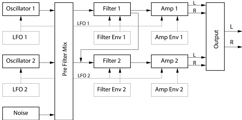
Diagram of Analog's Signal Flow.
