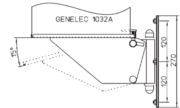
1032-460B Wall Mount
