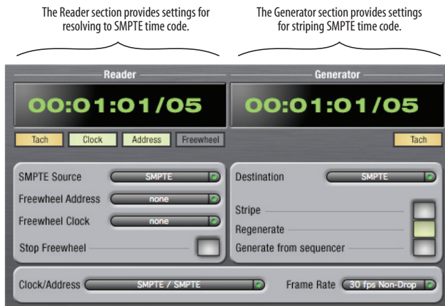
Figure 11-1: SMPTE Setup gives you access to your 828mk3's on-board SMPTE time code synchronization features.
