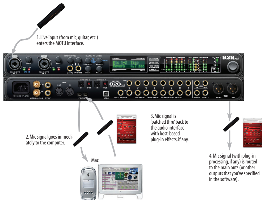
Figure 9-1: There are two ways to monitor live audio inputs with an 828mk3: 1) through the computer or 2) via CueMix FX hardware monitoring. This diagram shows method 1 (through the computer). When using this method, use your host software's buffer setting to reduce the slight delay you hear when monitoring the live input, but don't lower it too much, or your computer might get sluggish.
