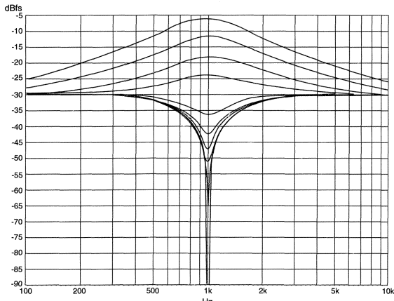
MPX 1 Parametric EQ: Gain
